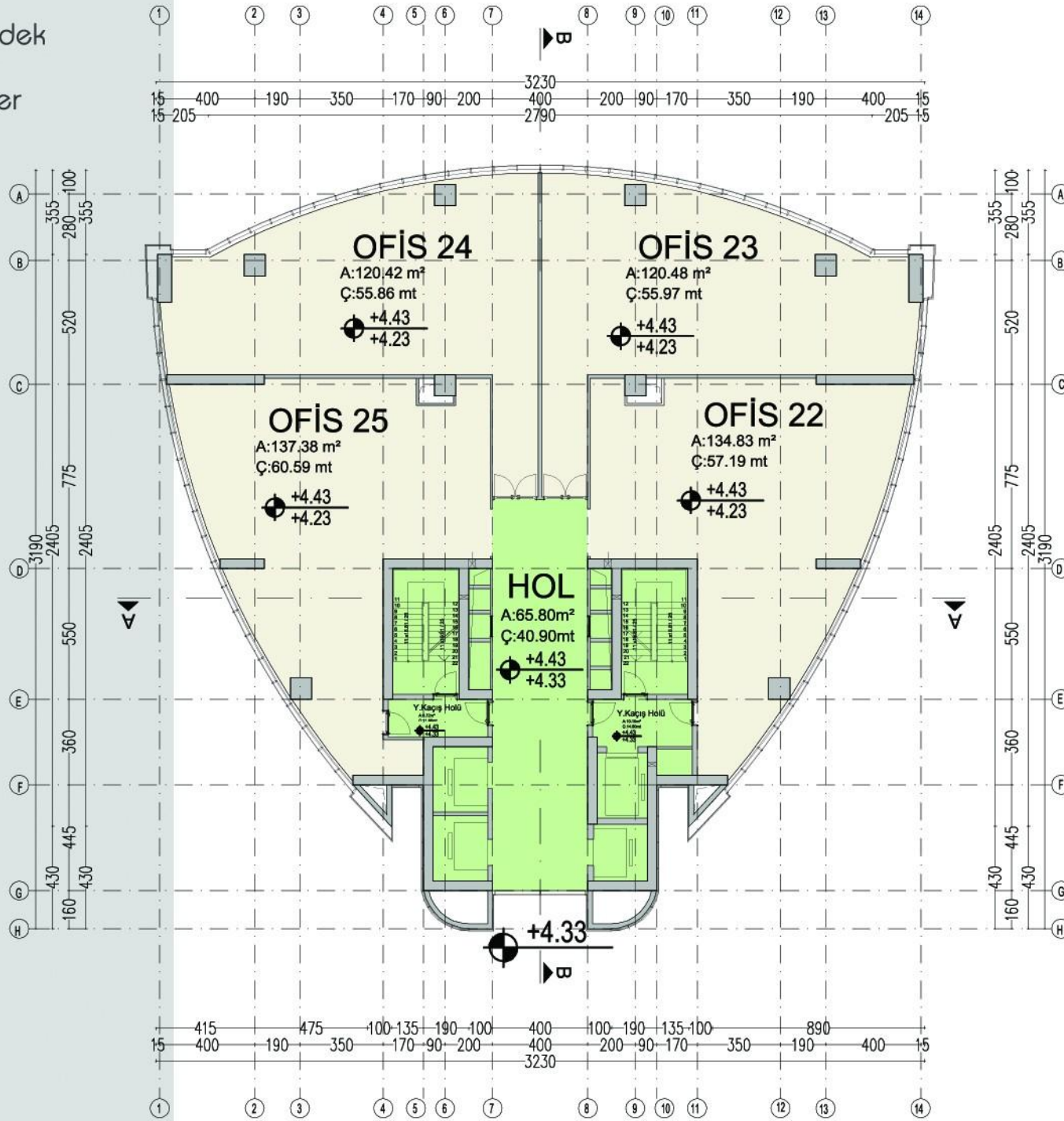
1. NORMAL KAT
