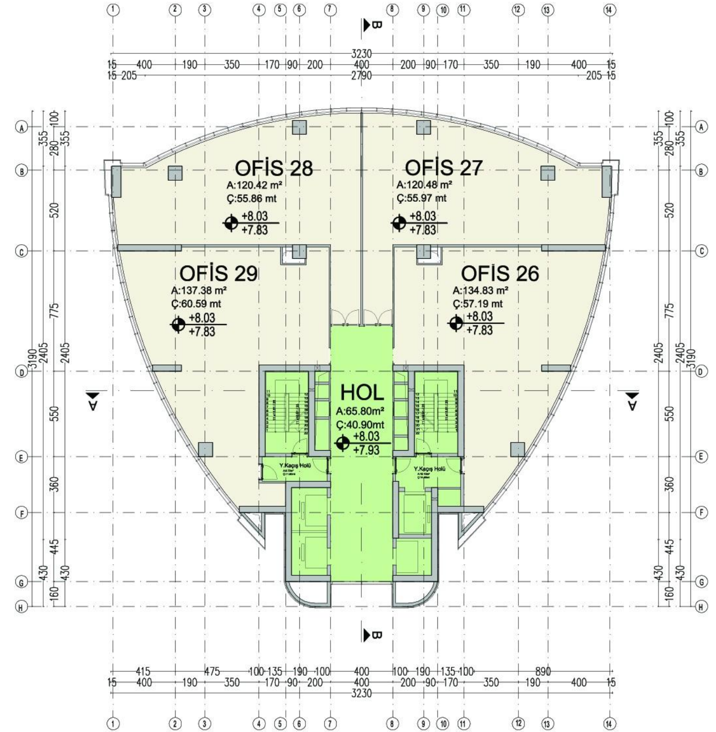
2. NORMAL KAT
